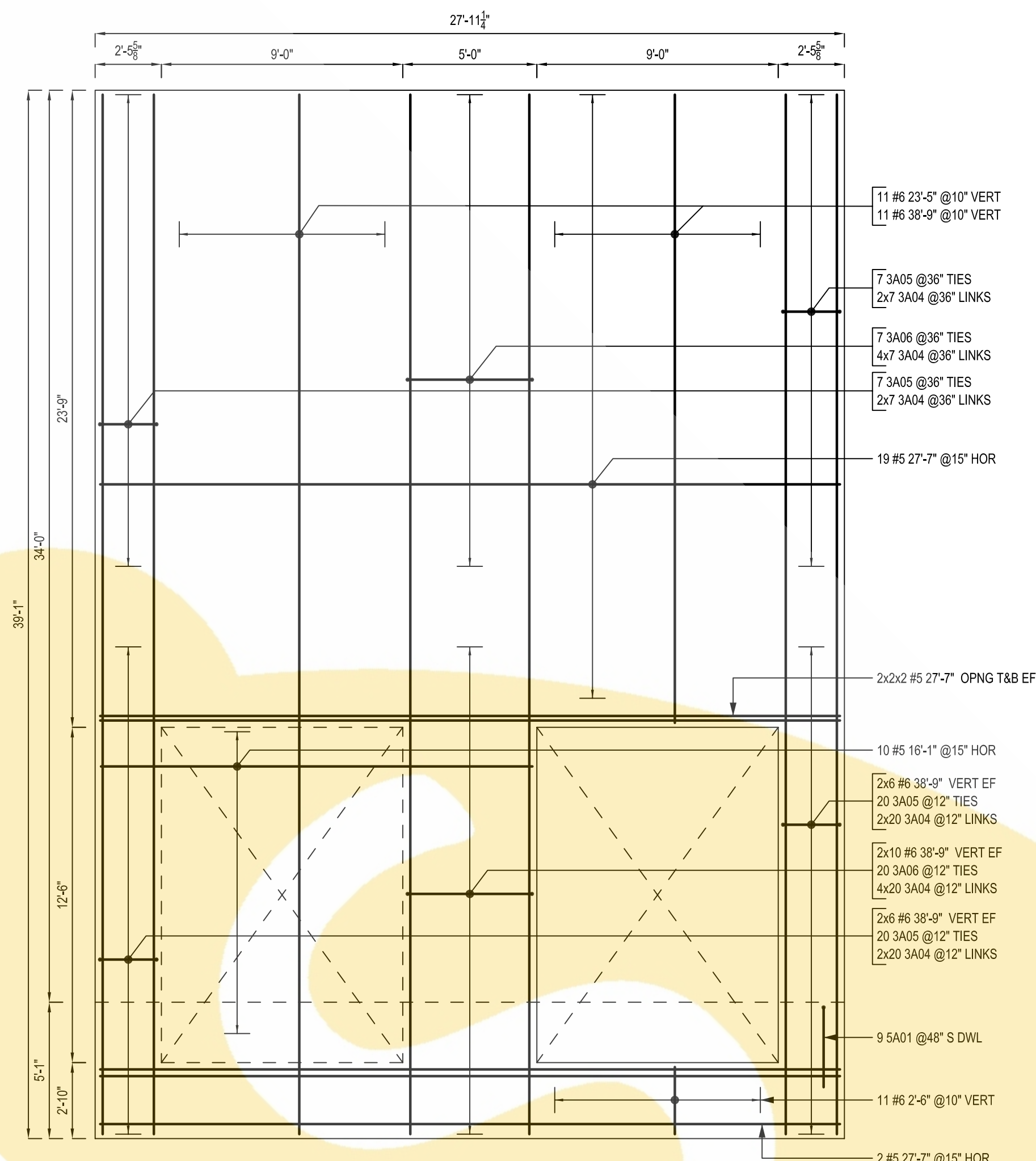
PANEL - N24 SCALE: 1/4"=1'-0" SDR: P18/T4.2
