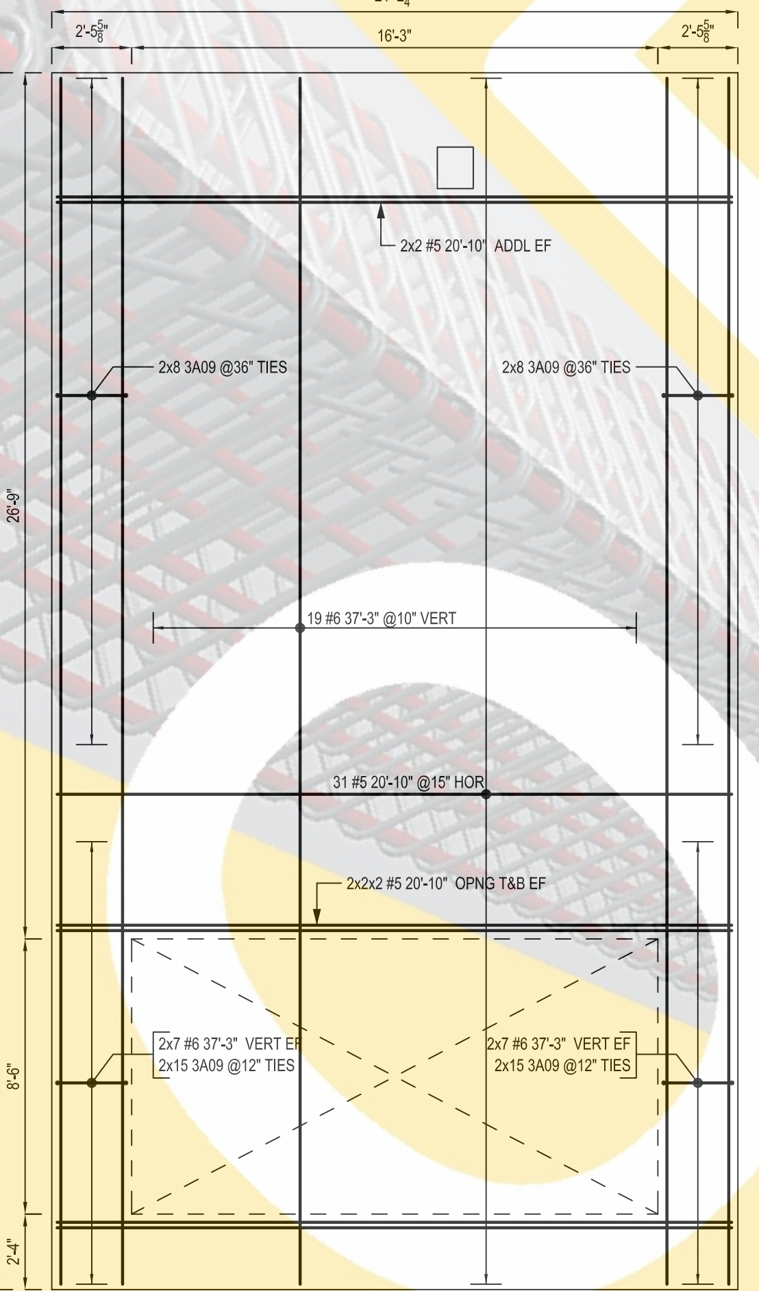
PANEL - W3 SCALE: 1/4"=1'-0" SDR: P3/T4.0
