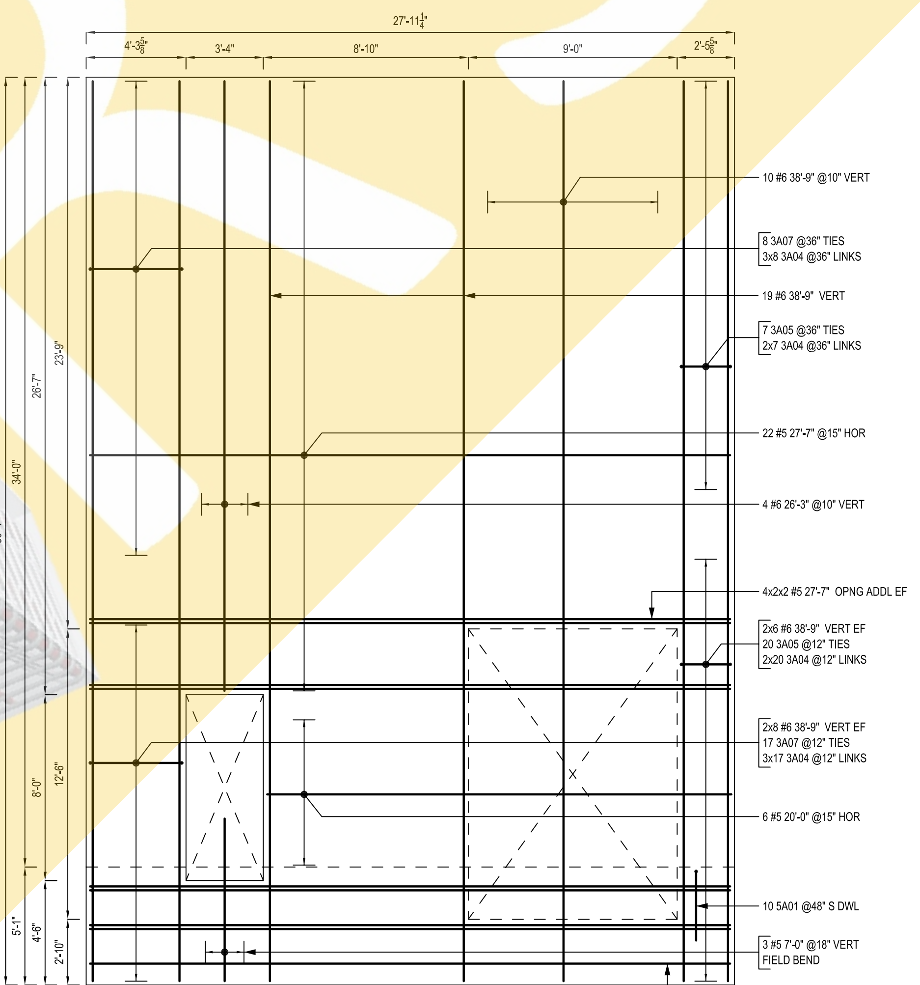
PANEL - N21 SCALE: 1/4"=1'-0" SDR: P16/T4.2
