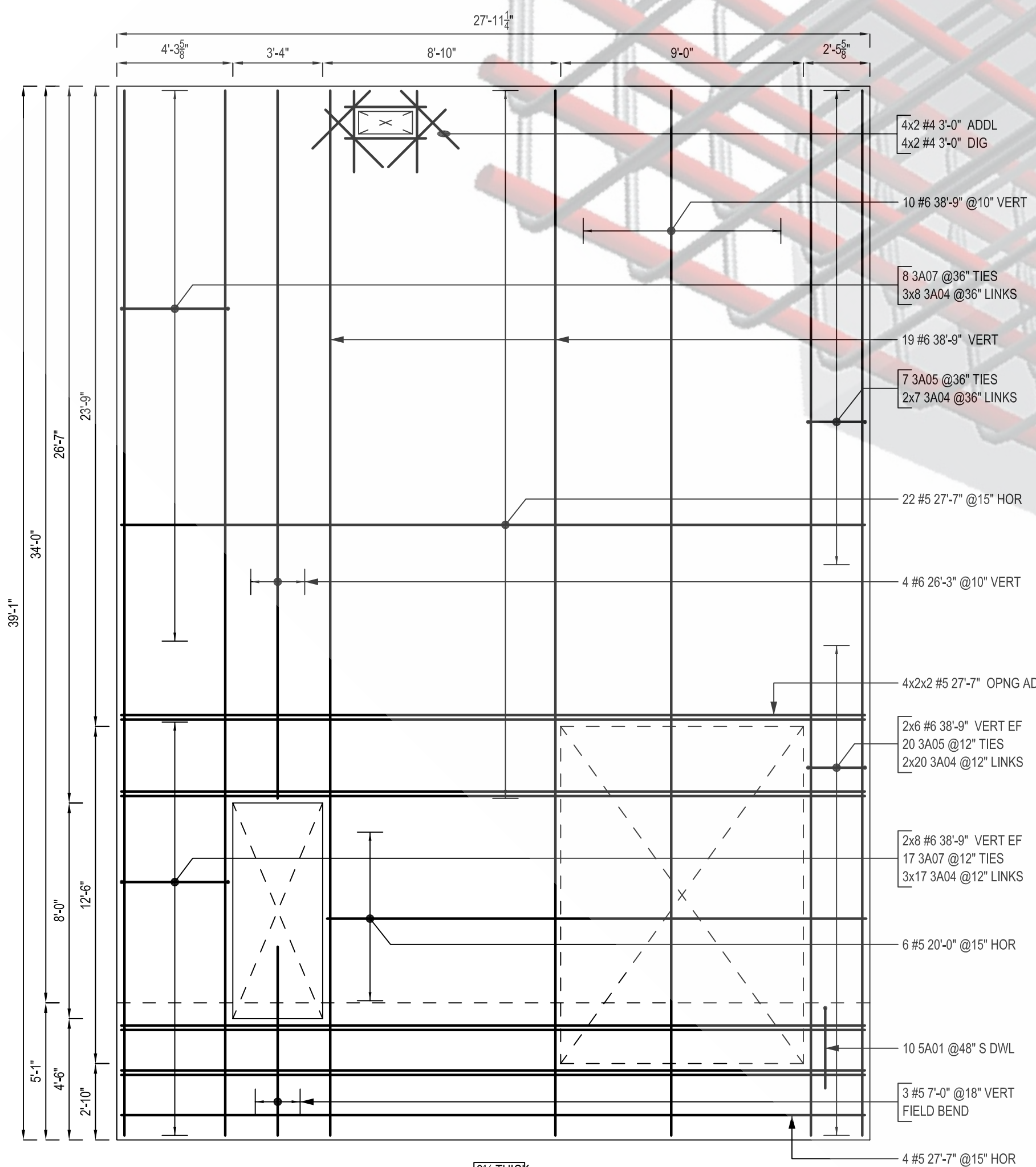
PANEL - N13 SCALE: 1/4"=1'-0" SDR: P18/T4.2
