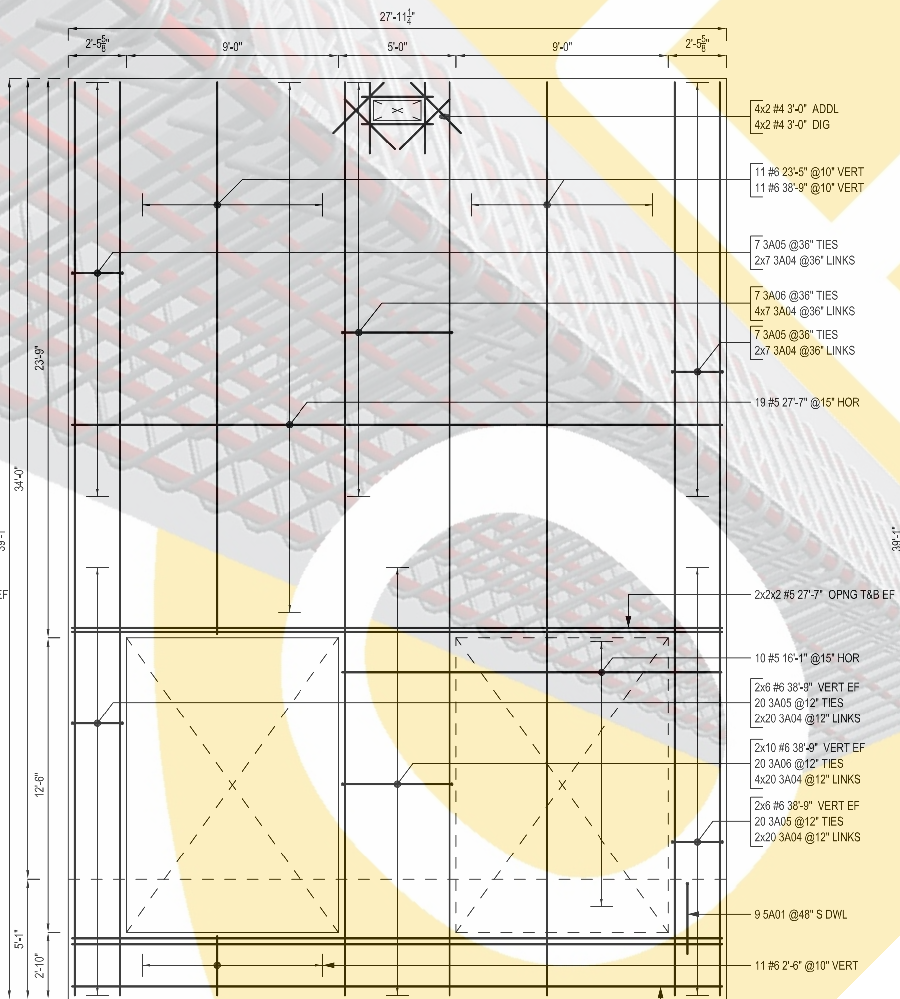
PANEL - N20 SCALE: 1/4"=1'-0" SDR: P16/T4.1
