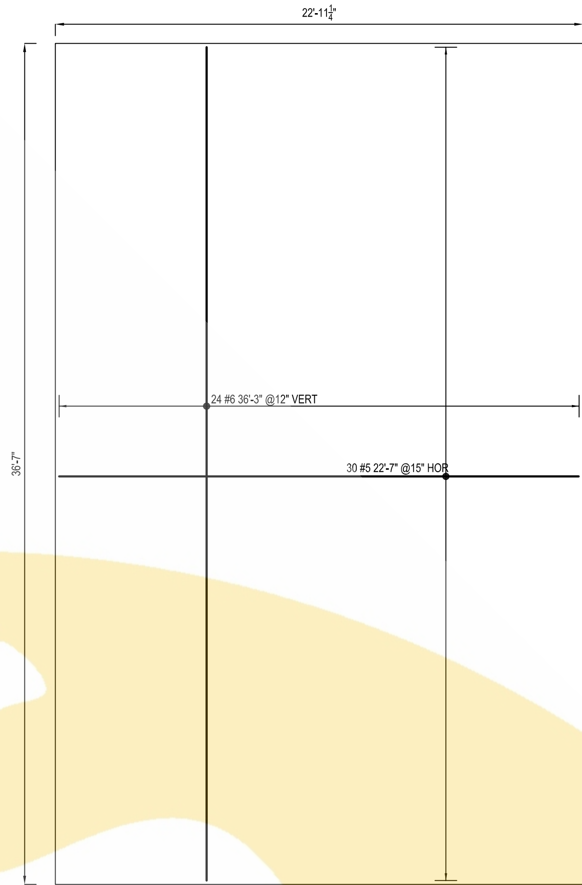
PANEL - S25 SCALE: 1/4"=1'-0" SDR: P34/T4.3
