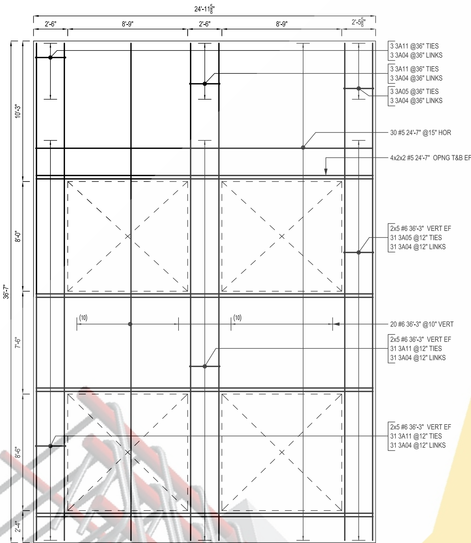
PANEL - S23 SCALE: 1/4"=1'-0" SDR: P30/T4.3
