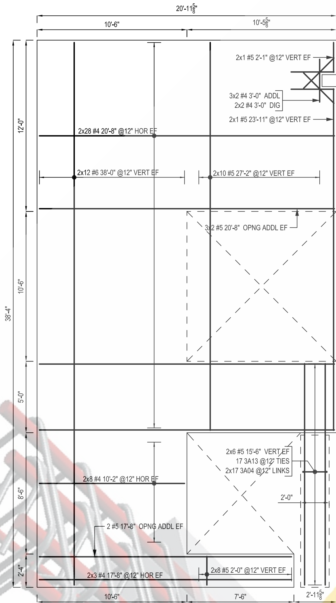
PANEL - S15 SCALE: 1/4"=1'-0" SDR: P22/T4.2
