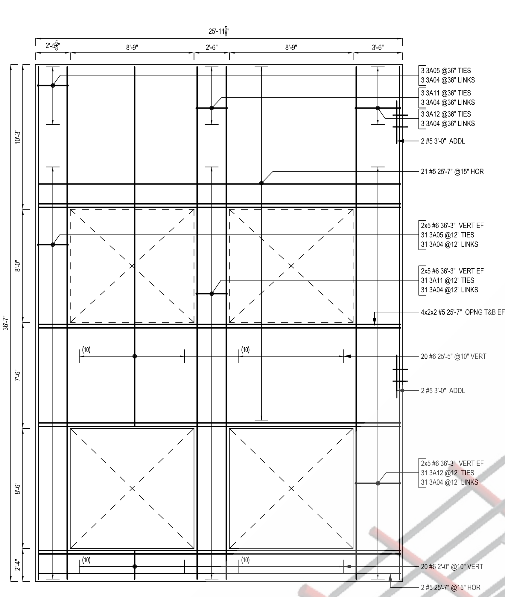
PANEL - S14 SCALE: 1/4"=1'-0" SDR: P32/T4.3
