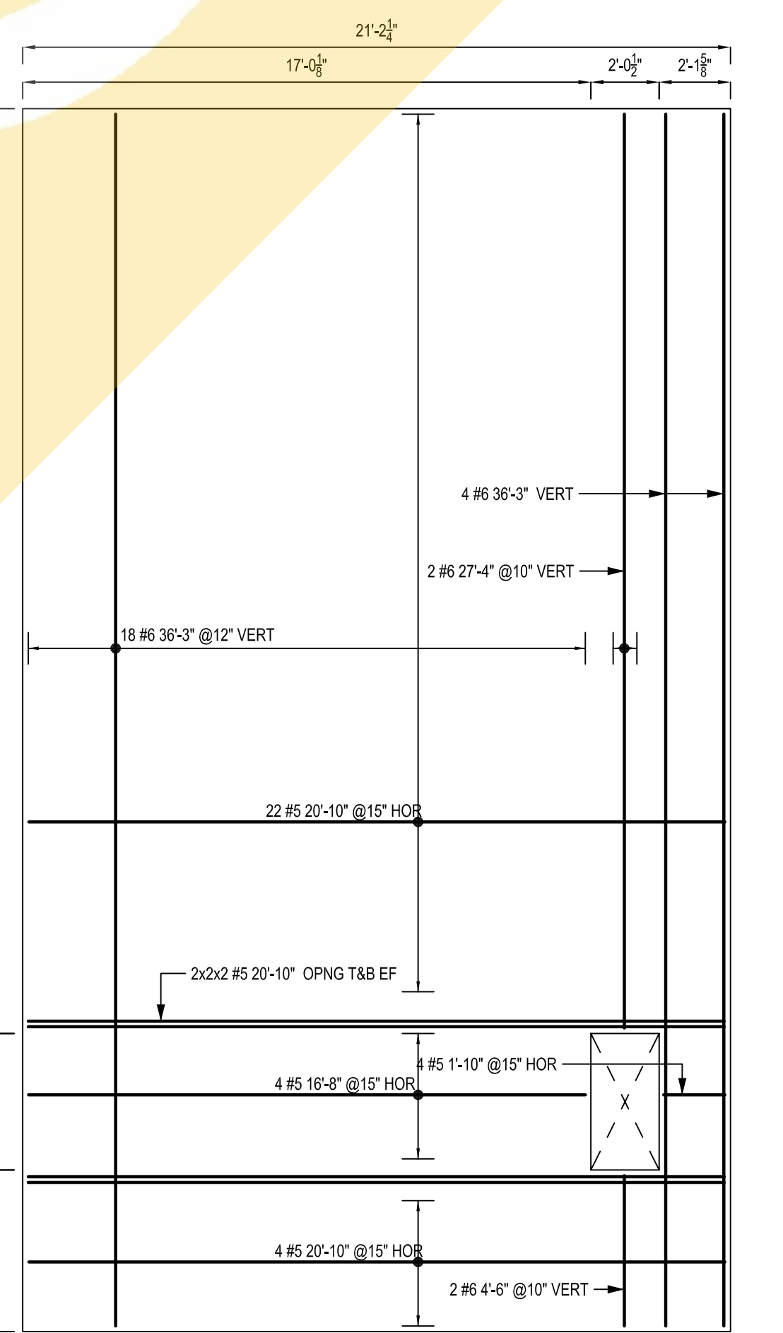
PANEL - W5 SCALE: 1/4"=1'-0" SDR: P5/T4.0
