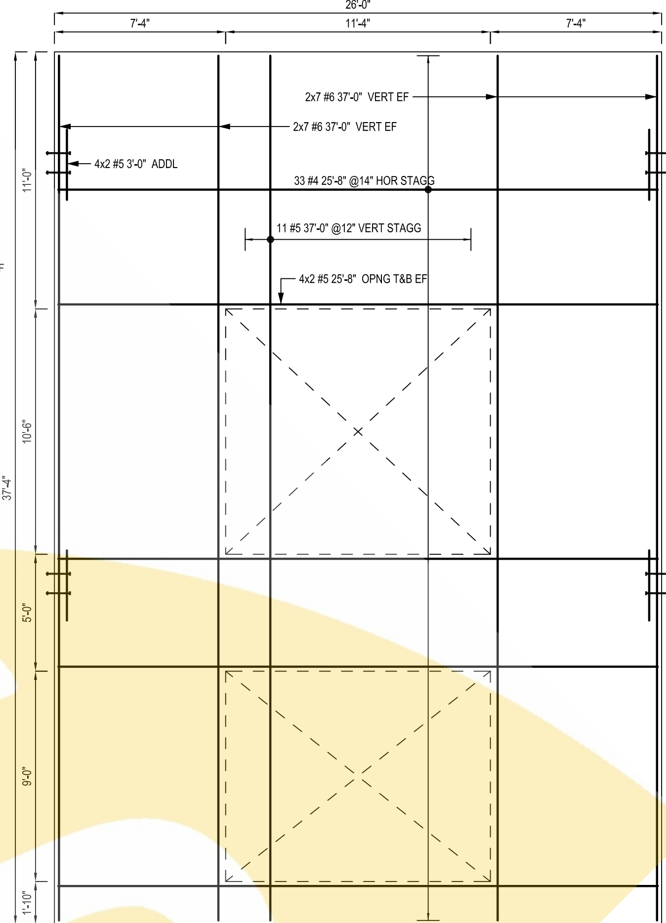
PANEL - S9 SCALE: 1/4"=1'-0" SDR: P29/T4.3
