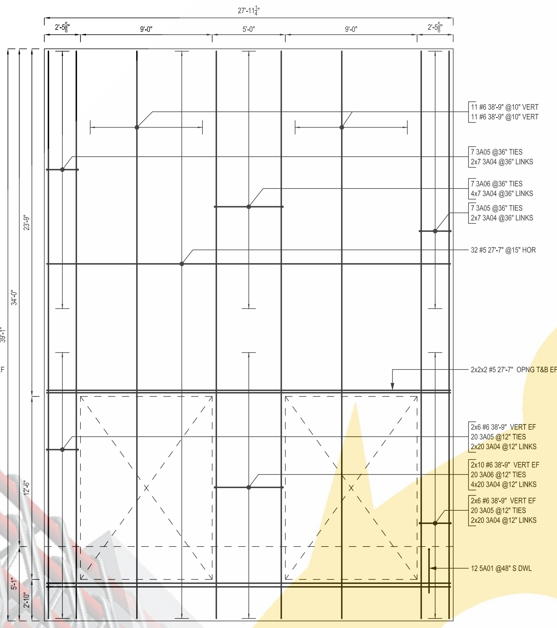
PANEL - N11 SCALE: 1/4"=1'-0" SDR: P17/T4.1
