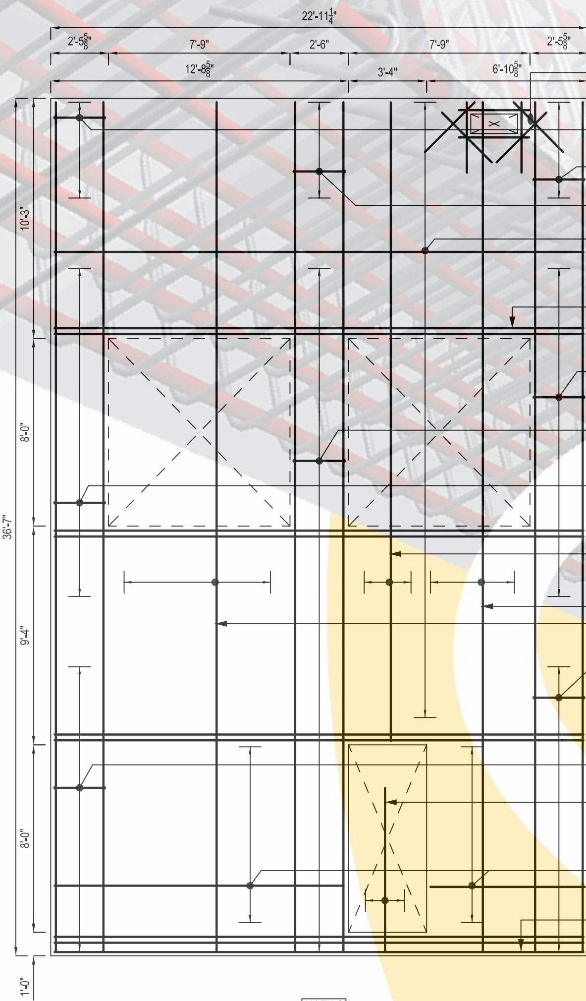
PANEL - S11 SCALE: 1/4"=1'-0" SDR: P31/T4.3
