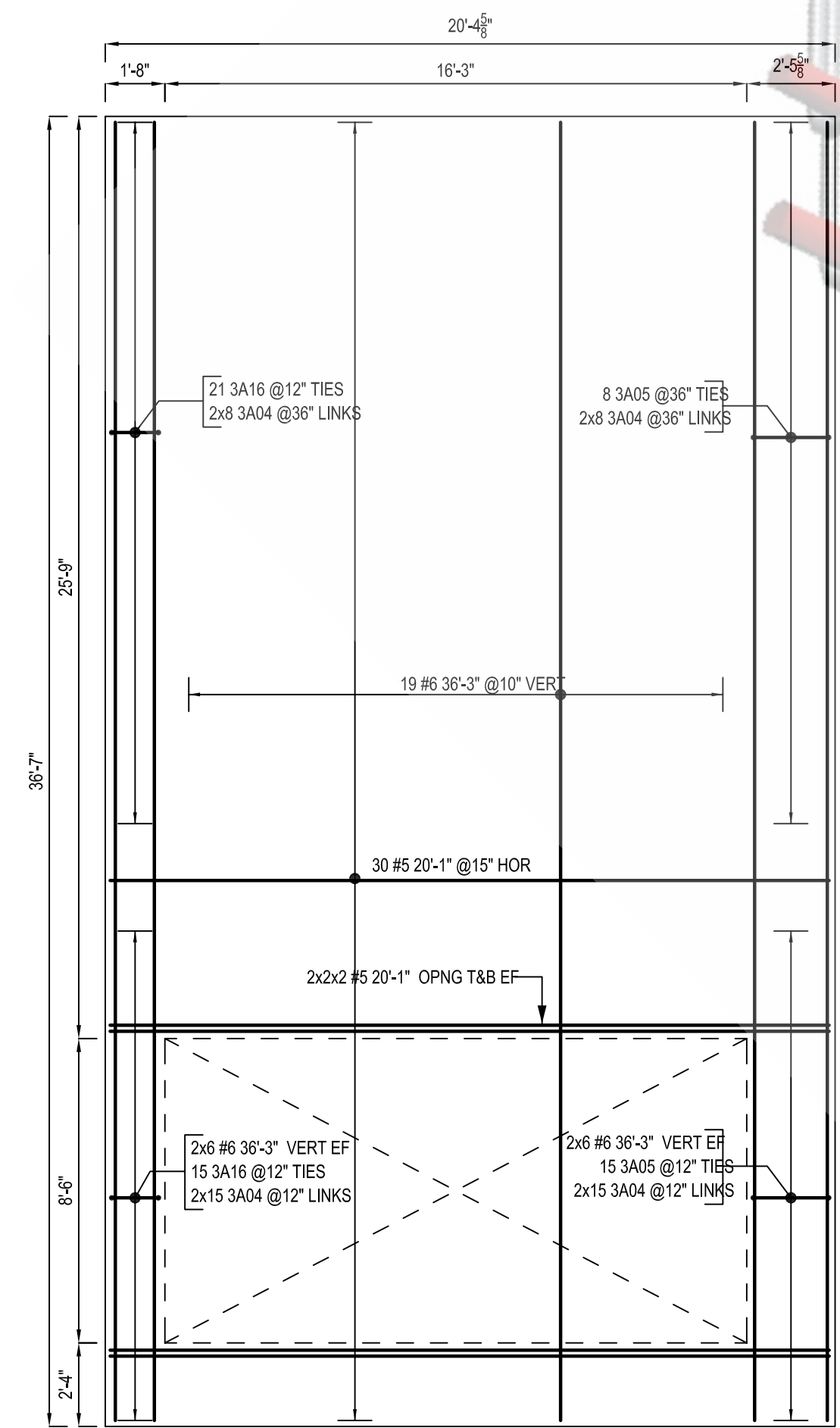
PANEL - W1 SCALE: 1/4"=1'-0" SDR: P1/T4.0
