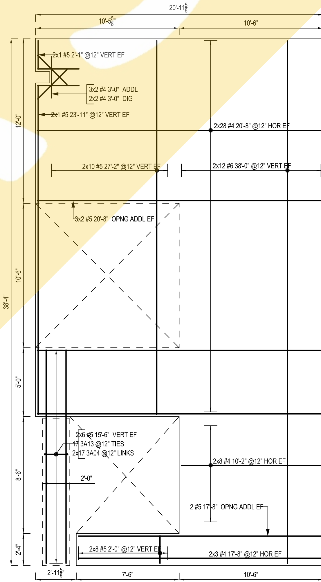
PANEL - S29 SCALE: 1/4"=1'-0" SDR: P23/T4.2
