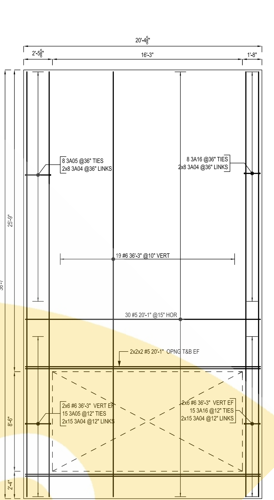
PANEL - E8 SCALE: 1/4"=1'-0" SDR: P4/T4.1
