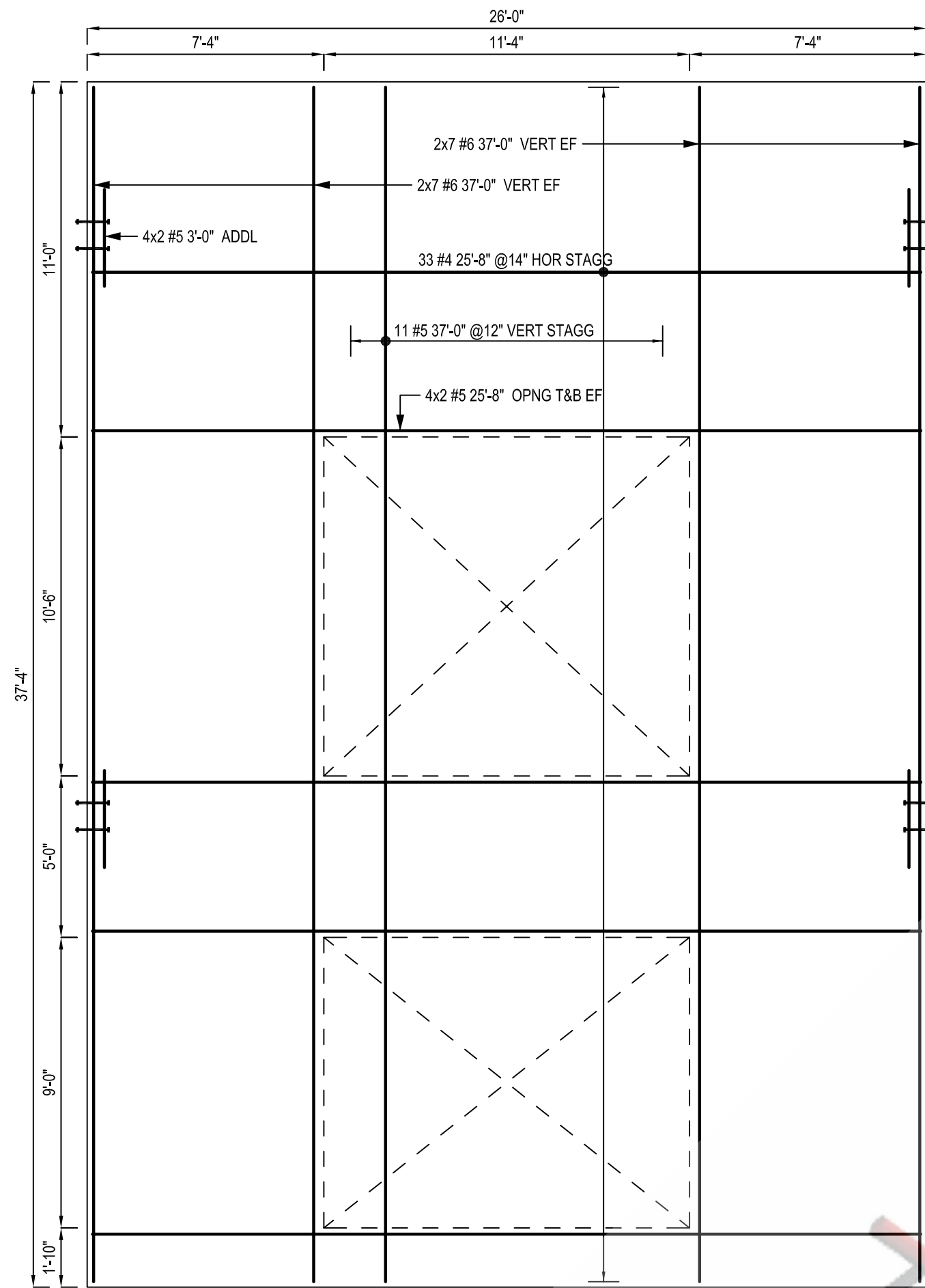
PANEL - S22 SCALE: 1/4"=1'-0" SDR: P29/T4.3
