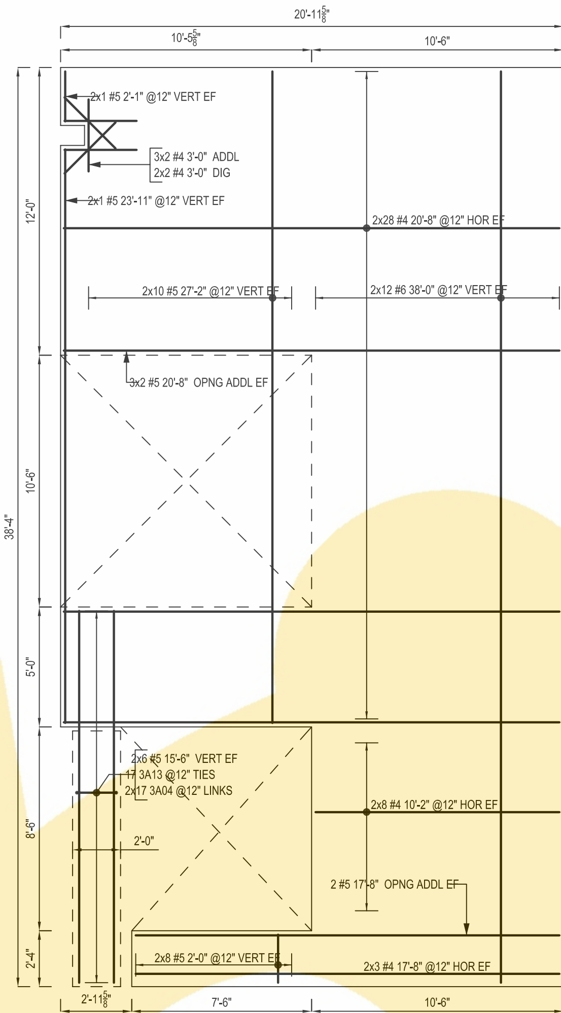
PANEL - S16 SCALE: 1/4"=1'-0" SDR: P23/T4.2
