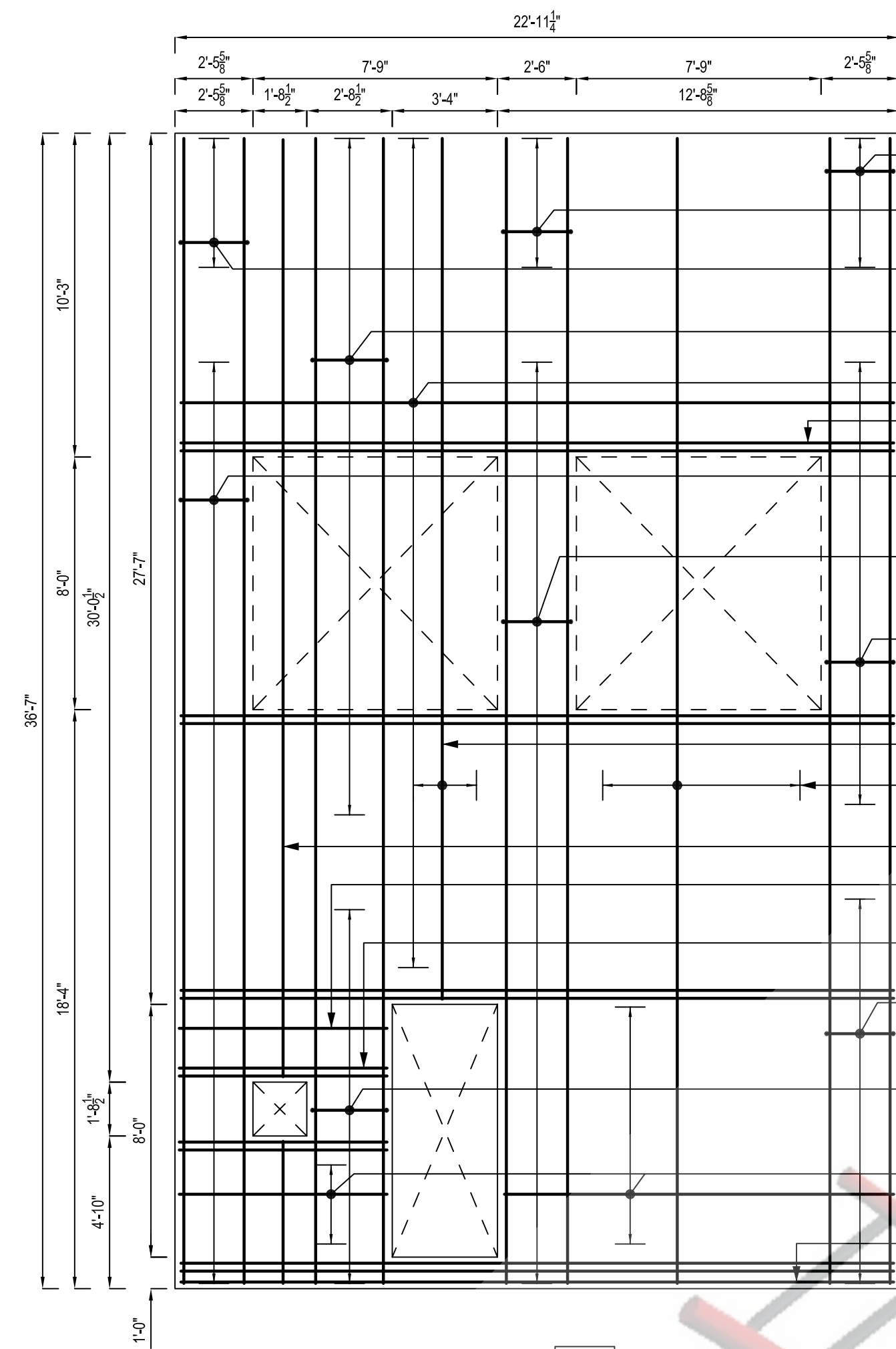
PANEL - S6 SCALE: 1/4"=1'-0" SDR: P26/T4.2
