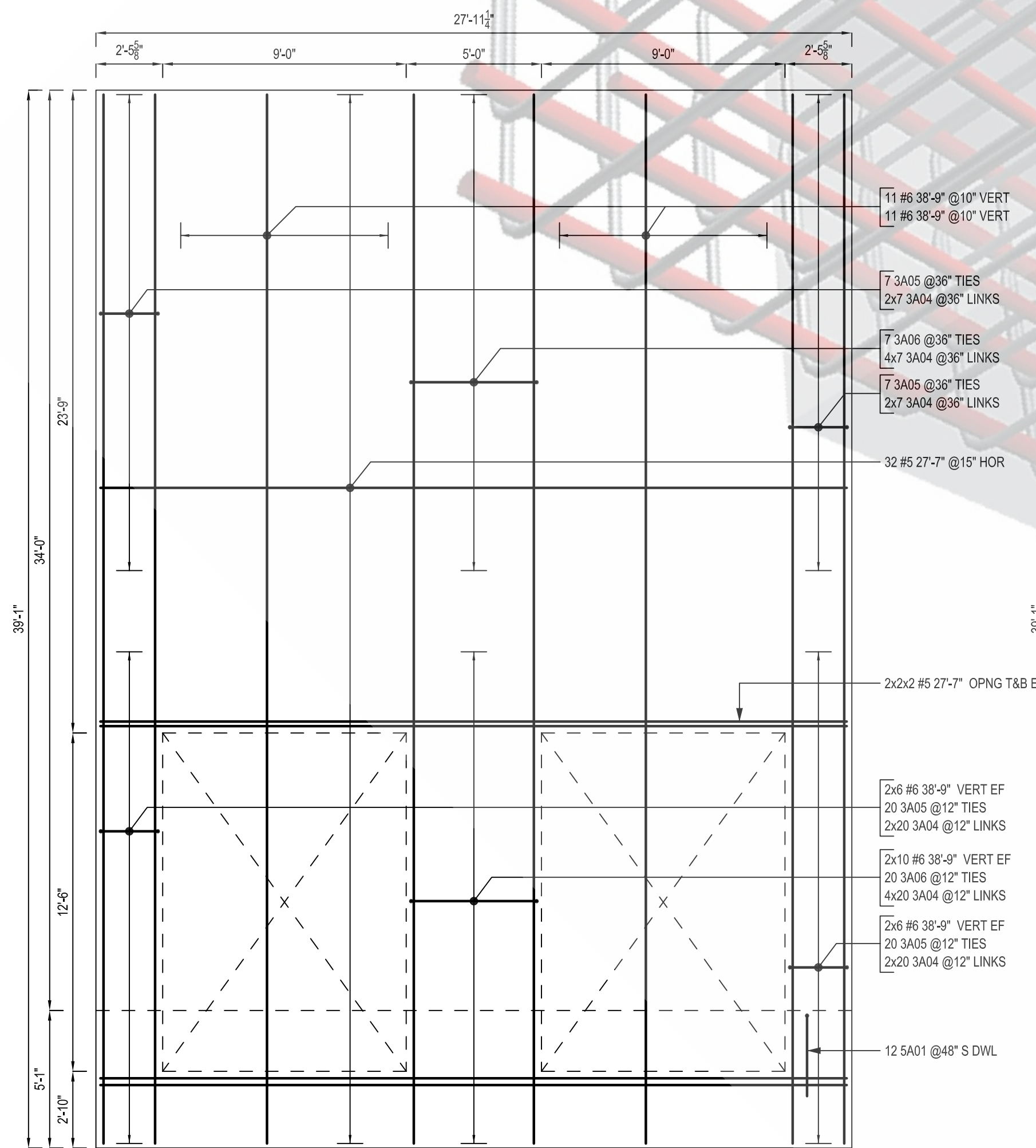
PANEL - N19 SCALE: 1/4"=1'-0" SDR: P17/T4.1
