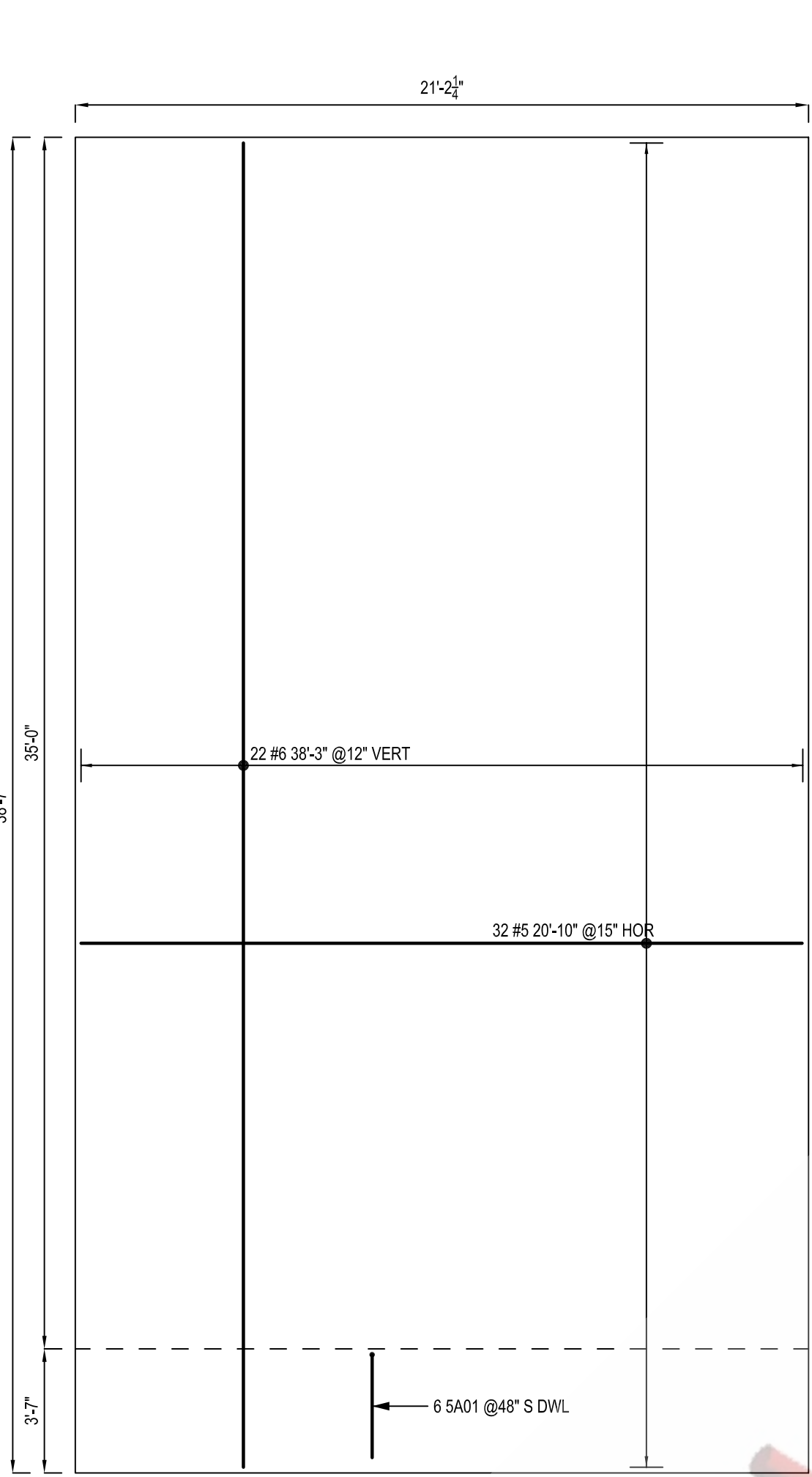
PANEL - E4 SCALE: 1/4"=1'-0" SDR: P11/T4.1
