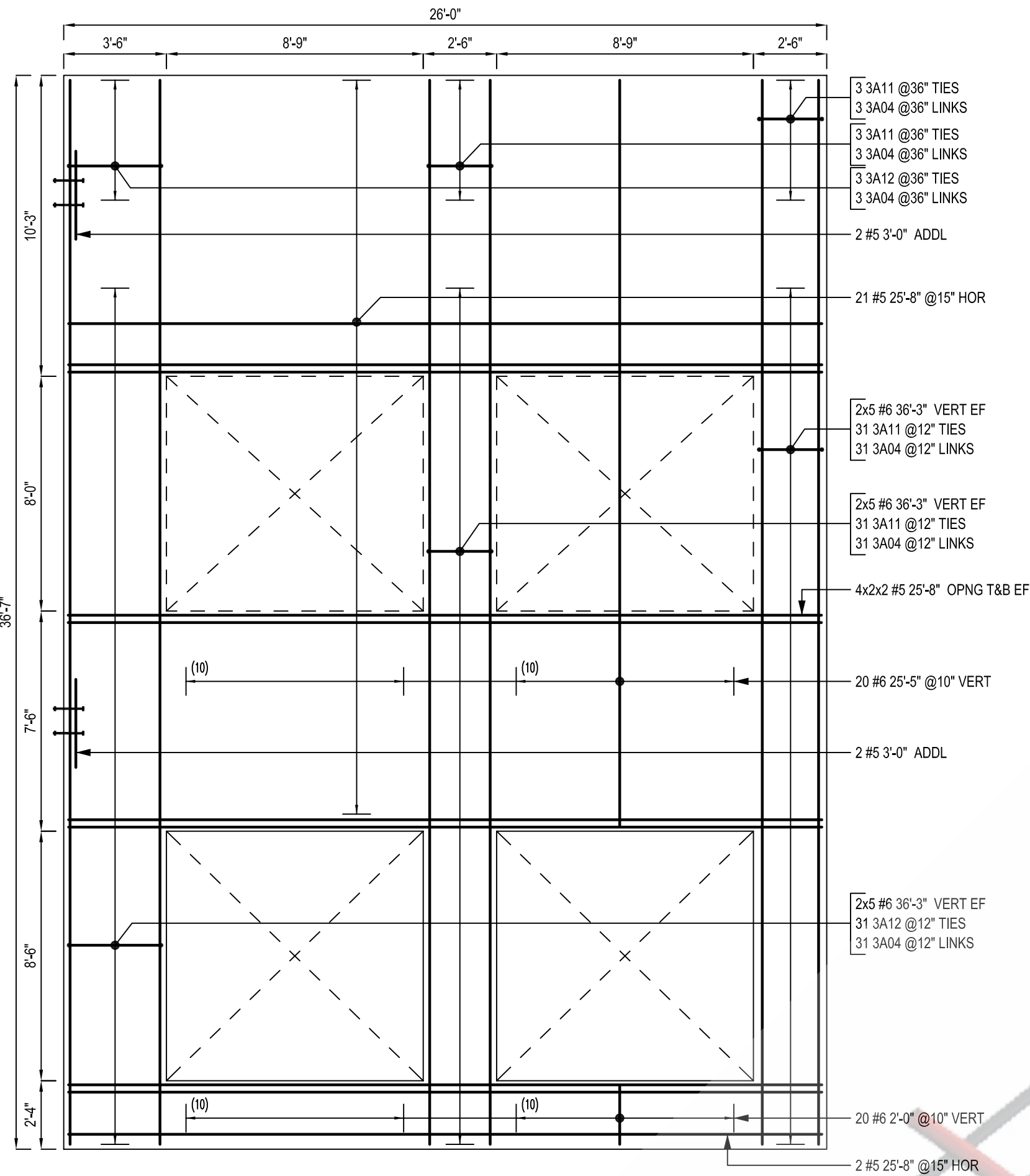
PANEL - S30 SCALE: 1/4"=1'-0" SDR: P35/T4.3
