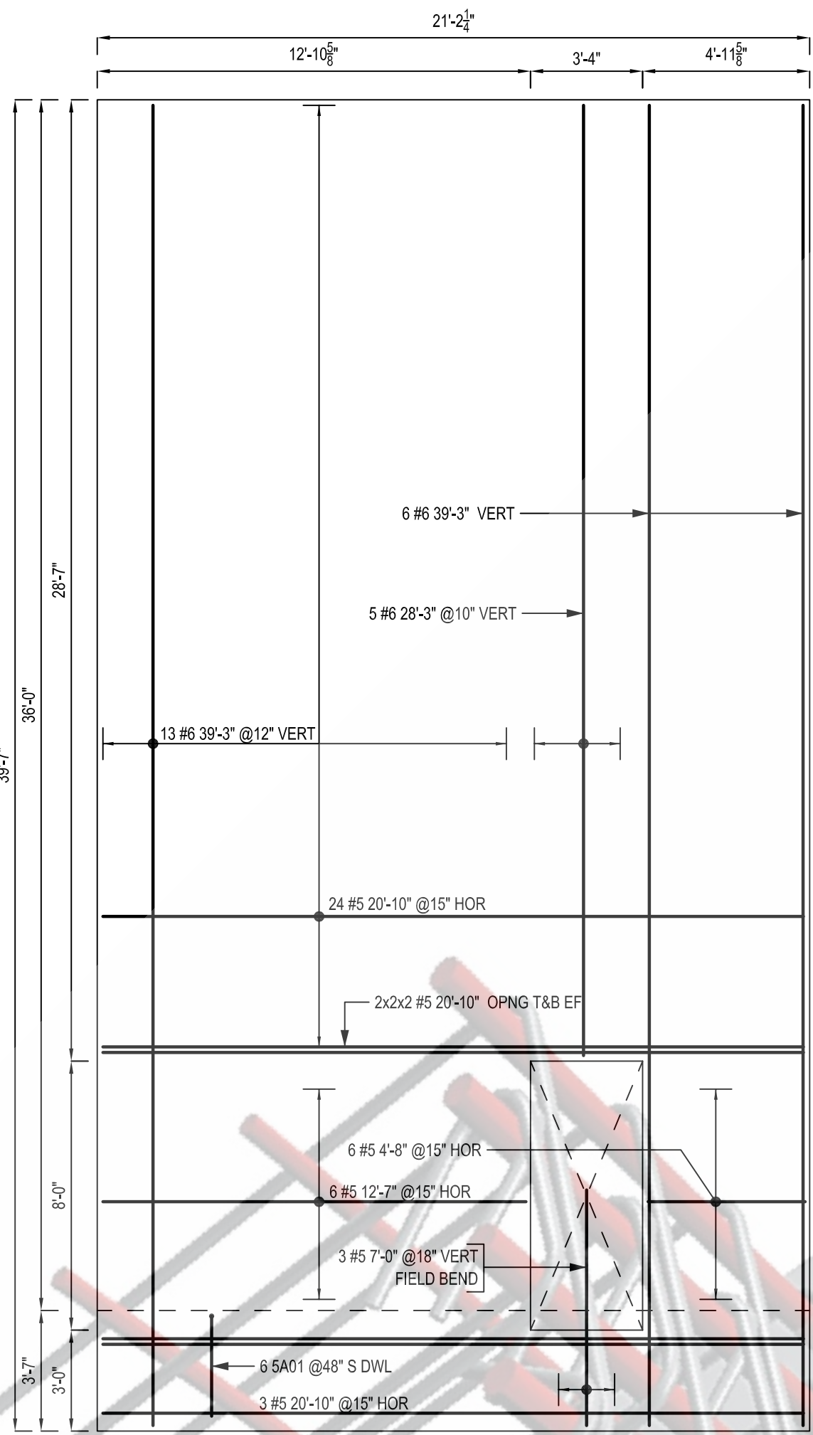
PANEL - E5 SCALE: 1/4"=1'-0" SDR: P12/T4.1
