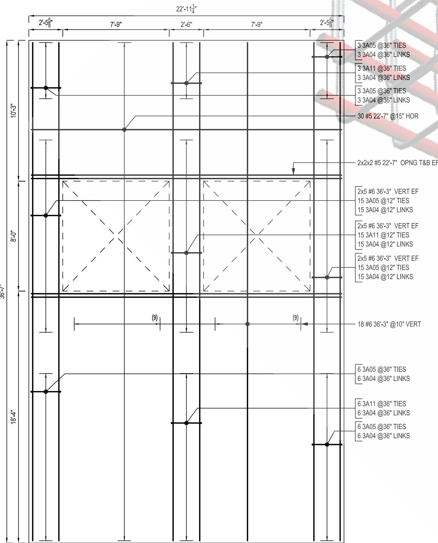
PANEL - S18 SCALE: 1/4"=1'-0" SDR: P25/T4.2
