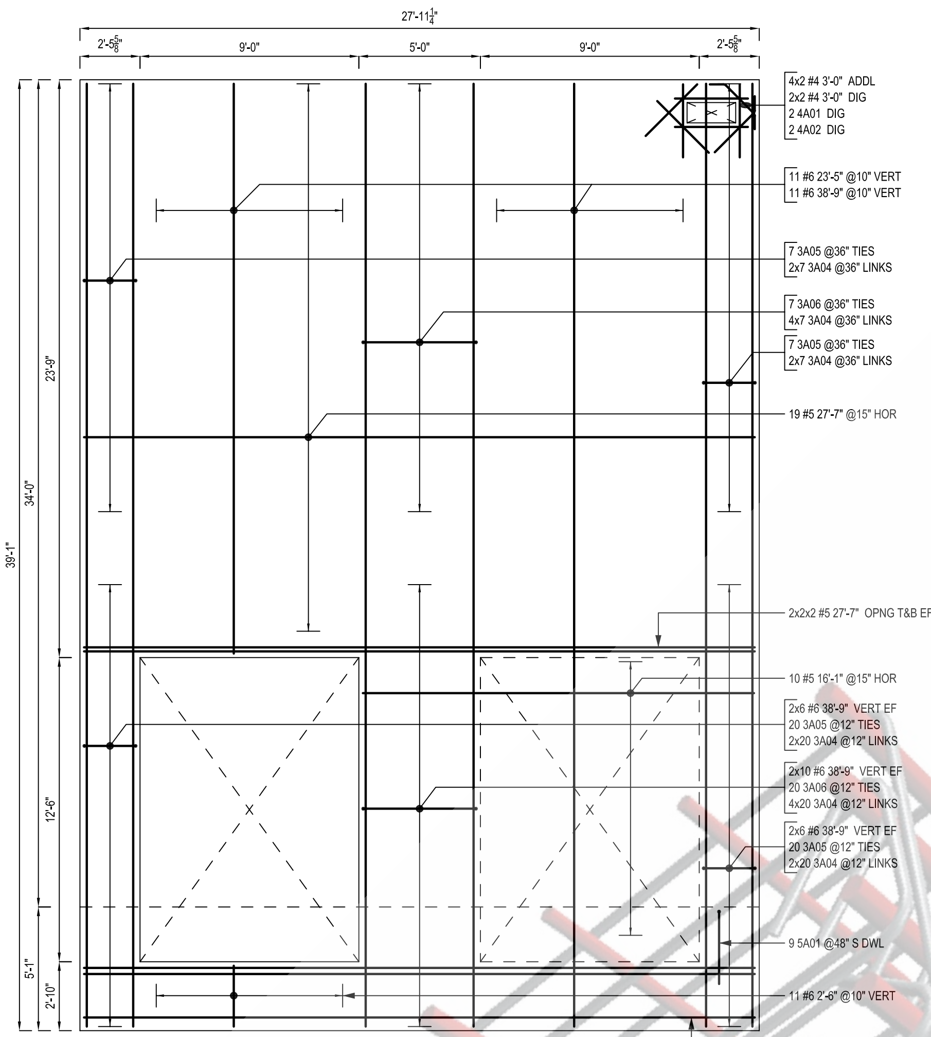
PANEL - N16 SCALE: 1/4"=1'-0" SDR: P16/T4.1
