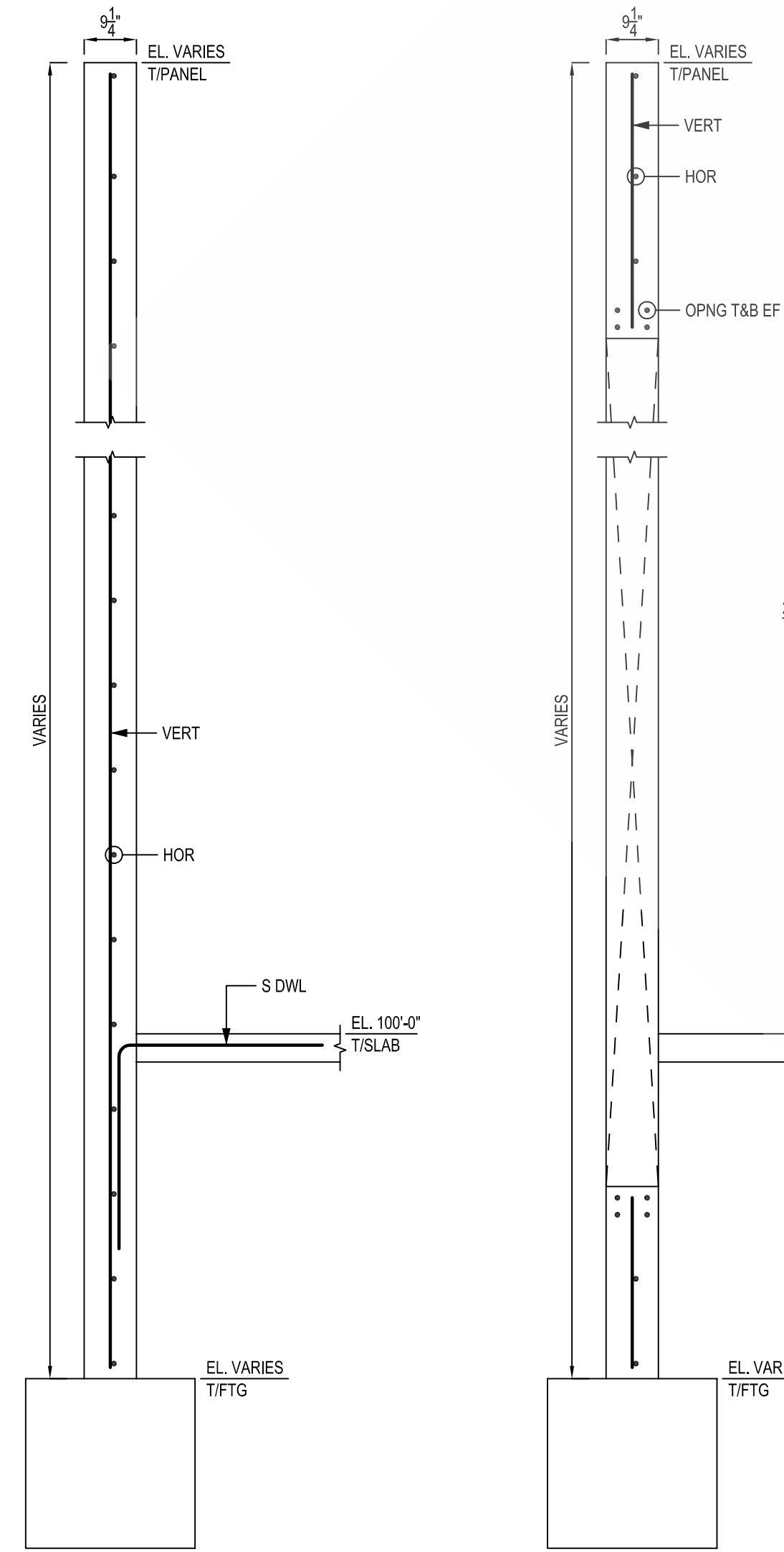
TYPICAL DETAIL SCALE: 1/2"=1'-0"
