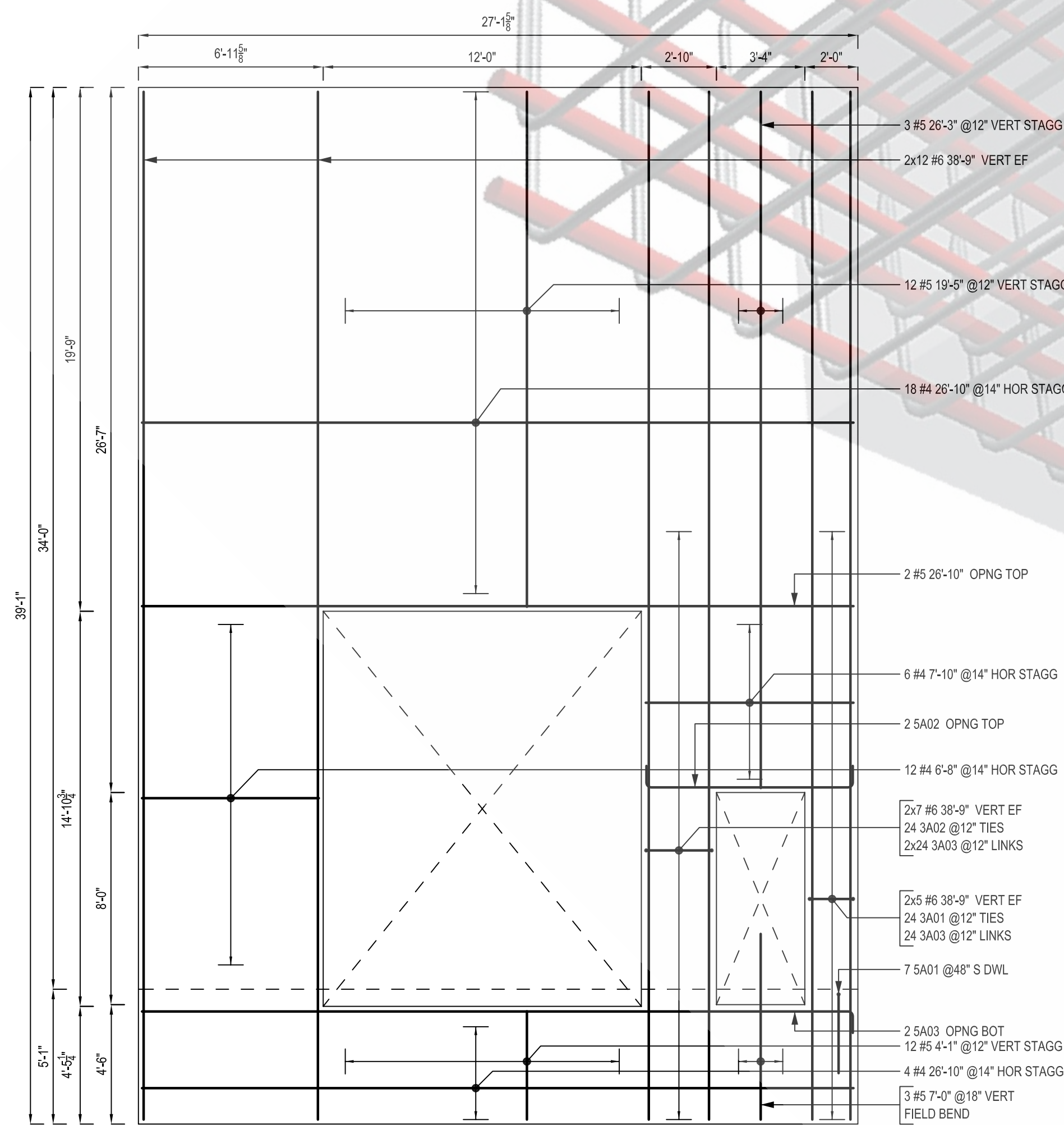
PANEL - N25 SCALE: 1/4"=1'-0" SDR: P20/T4.2
