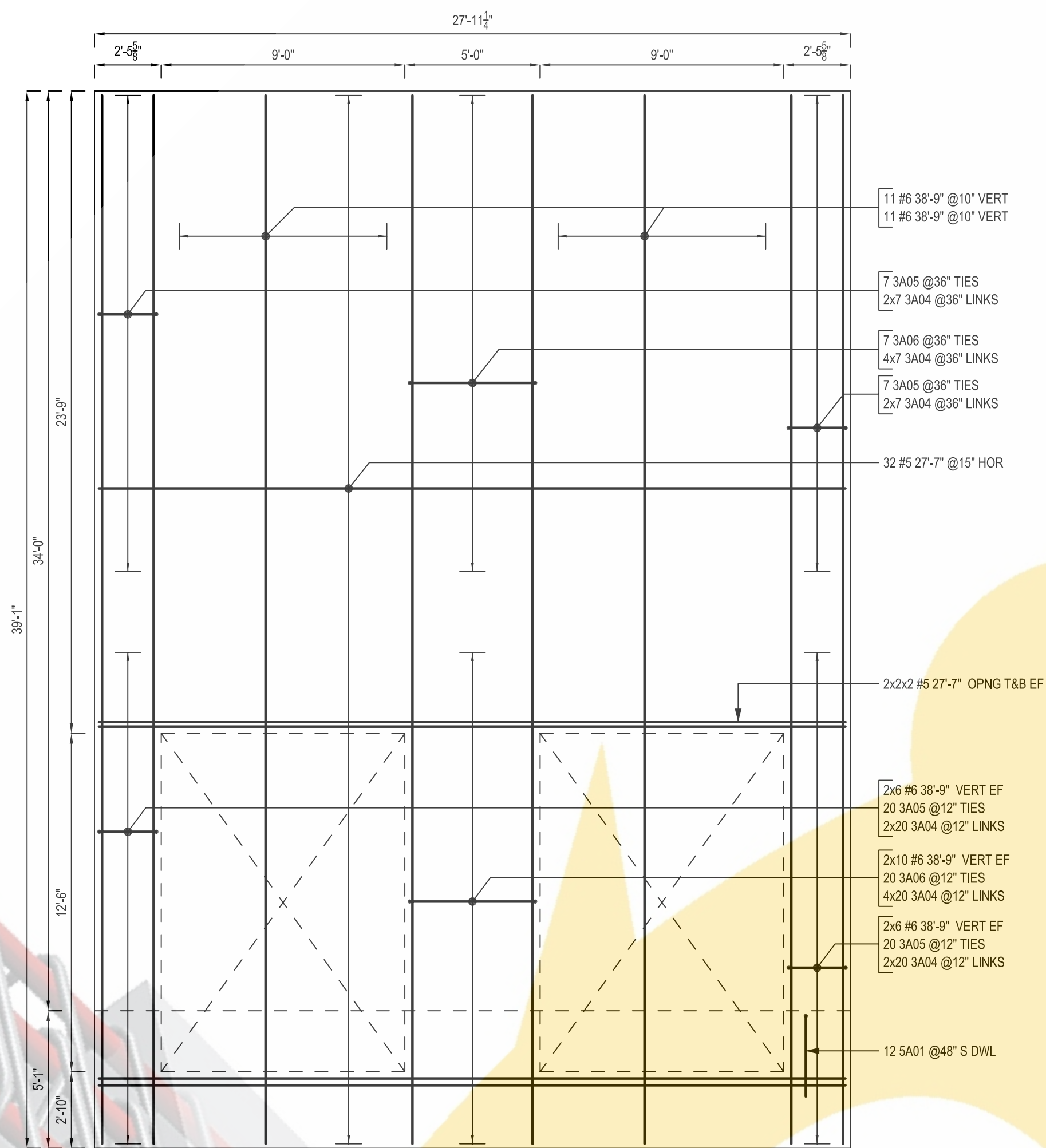
PANEL - N23 SCALE: 1/4"=1'-0" SDR: P17/T4.1
