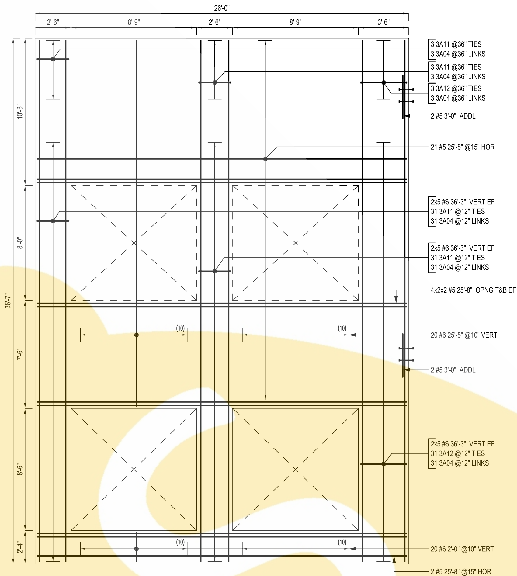
PANEL - S1 SCALE: 1/4"=1'-0" SDR: P21/T4.2
