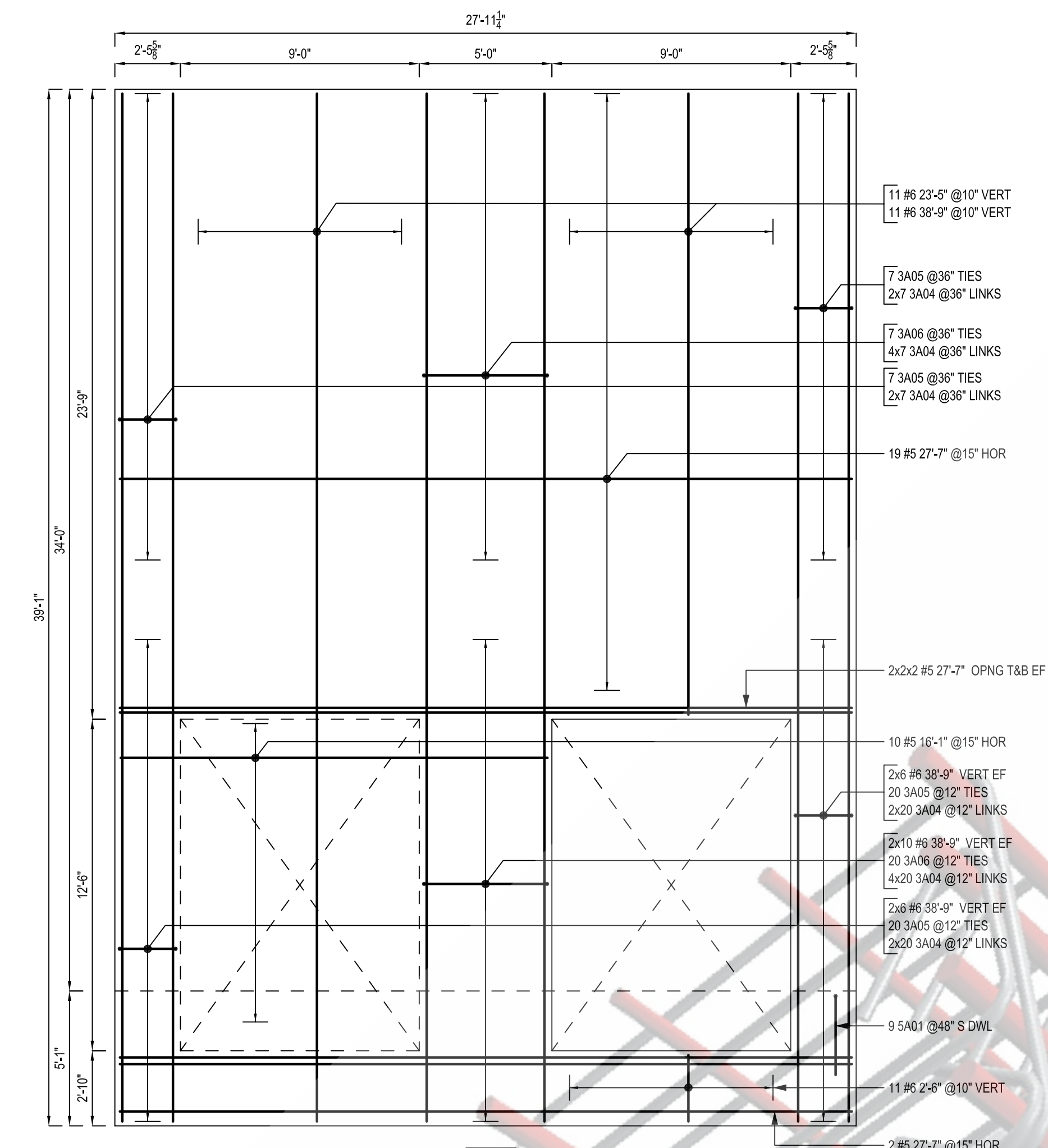
PANEL - N22 SCALE: 1/4"=1'-0" SDR: P19/T4.2
