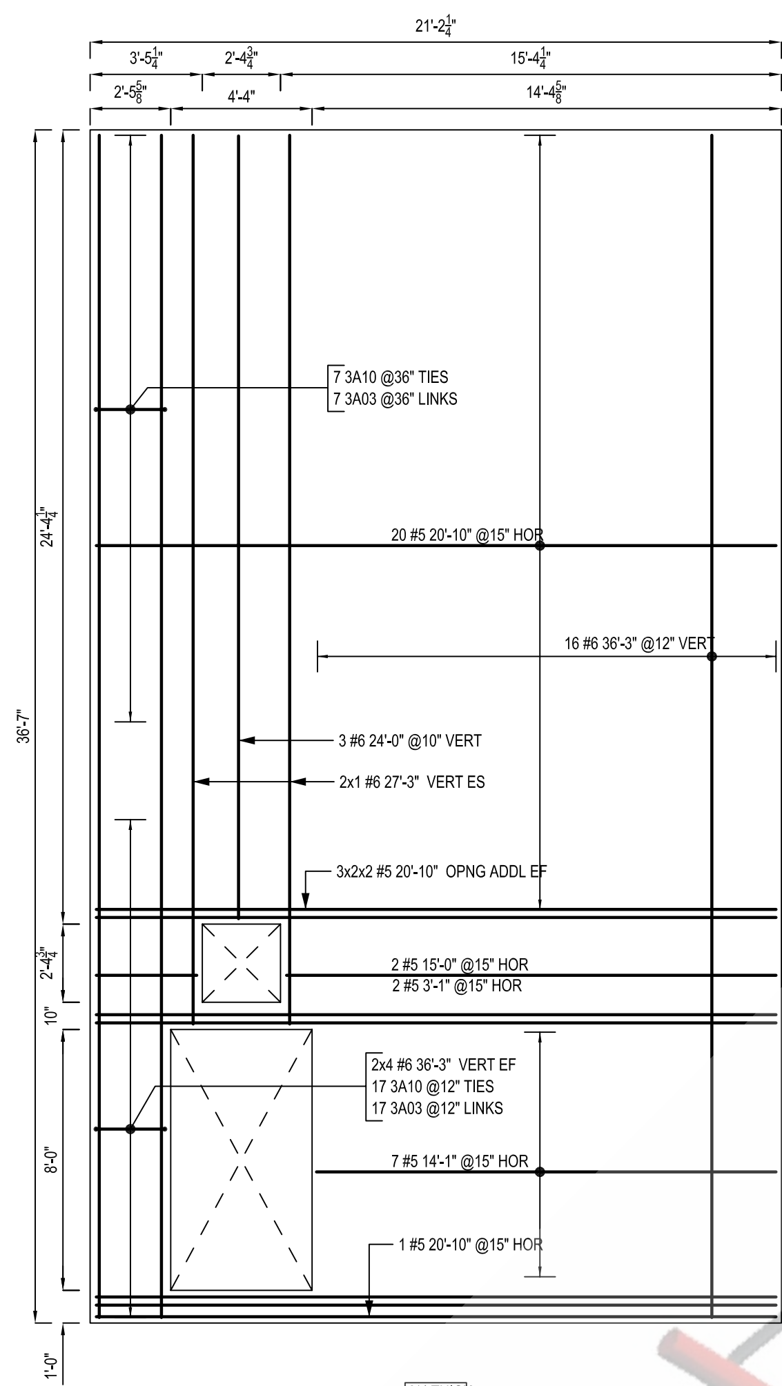
PANEL - W6 SCALE: 1/4"=1'-0" SDR: P6/T4.0
