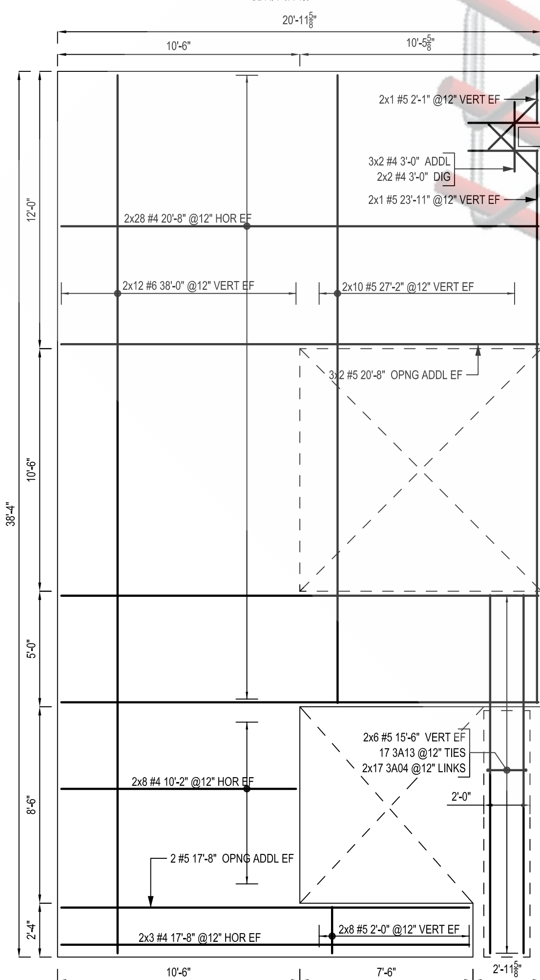
PANEL - S2 SCALE: 1/4"=1'-0" SDR: P22/T4.2
