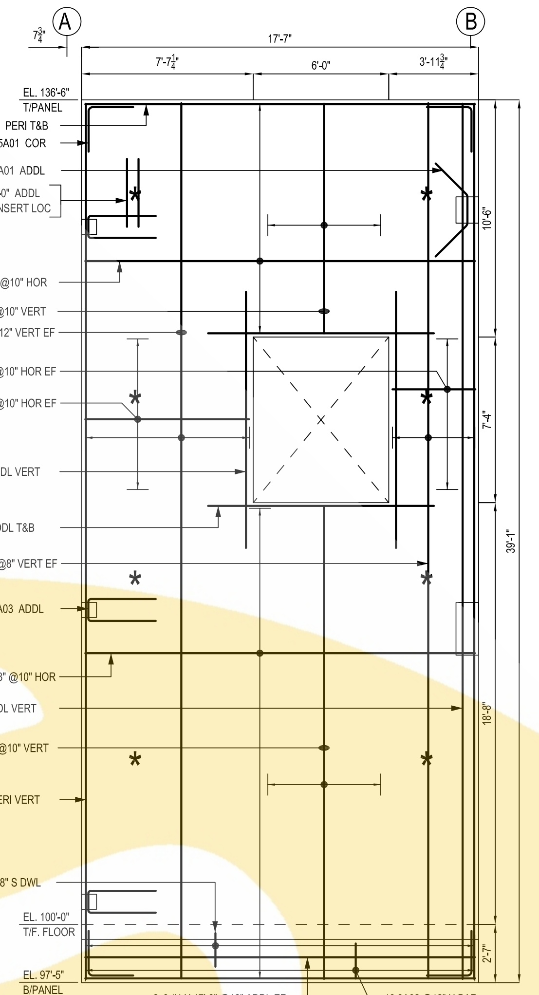
PANEL-P8 SCALE: 1/4"=1'-0" SDR: S2.01 & S3.11
