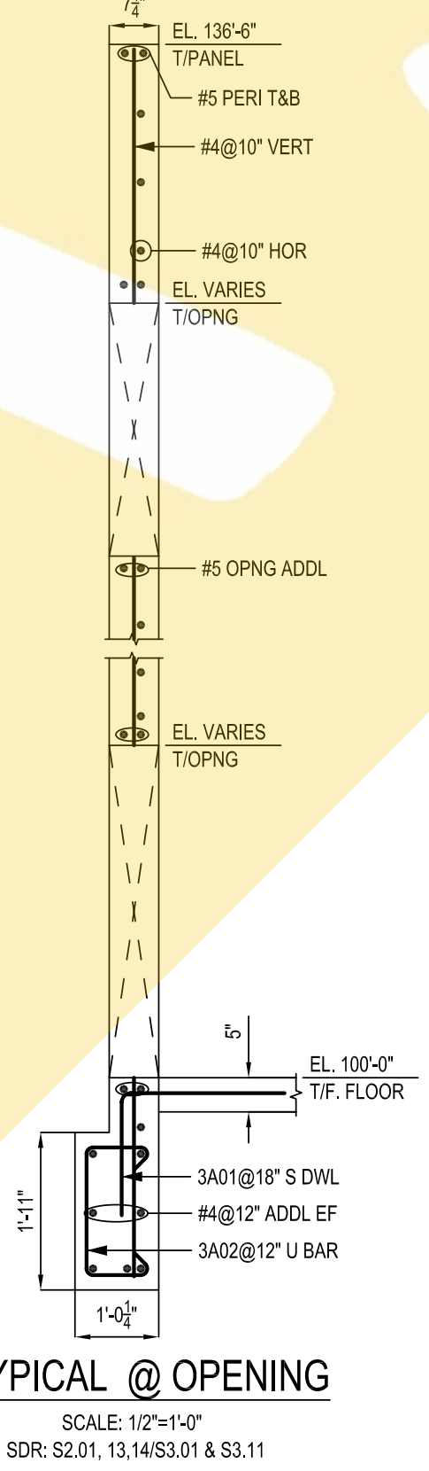
TYPICAL DETAIL SCALE: 1/2"=1'-0" SDR: S2.01, 12B/S3.01 & S3.11
