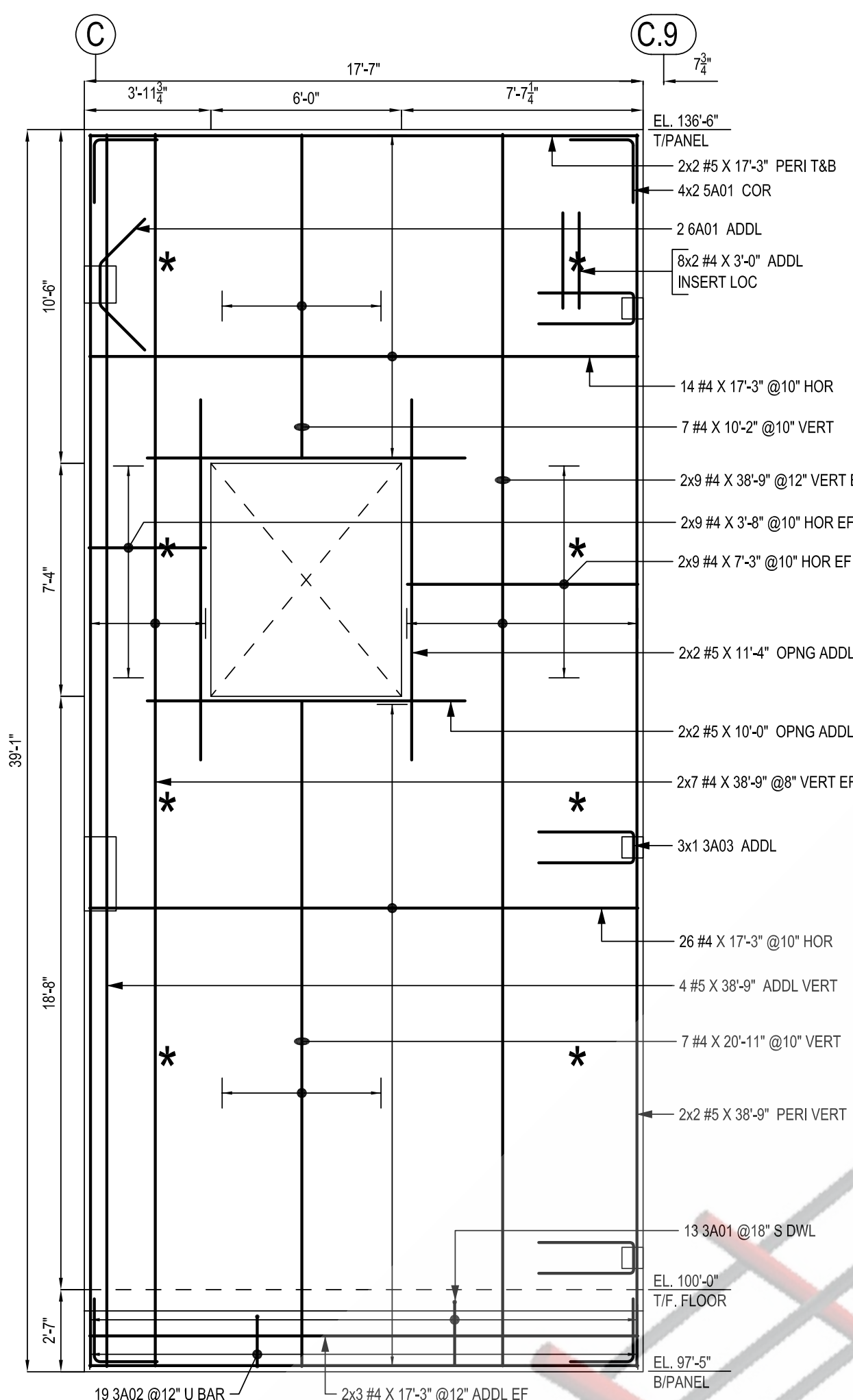
PANEL-P6 SCALE: 1/4"=1'-0" SDR: S2.01 & S3.11
