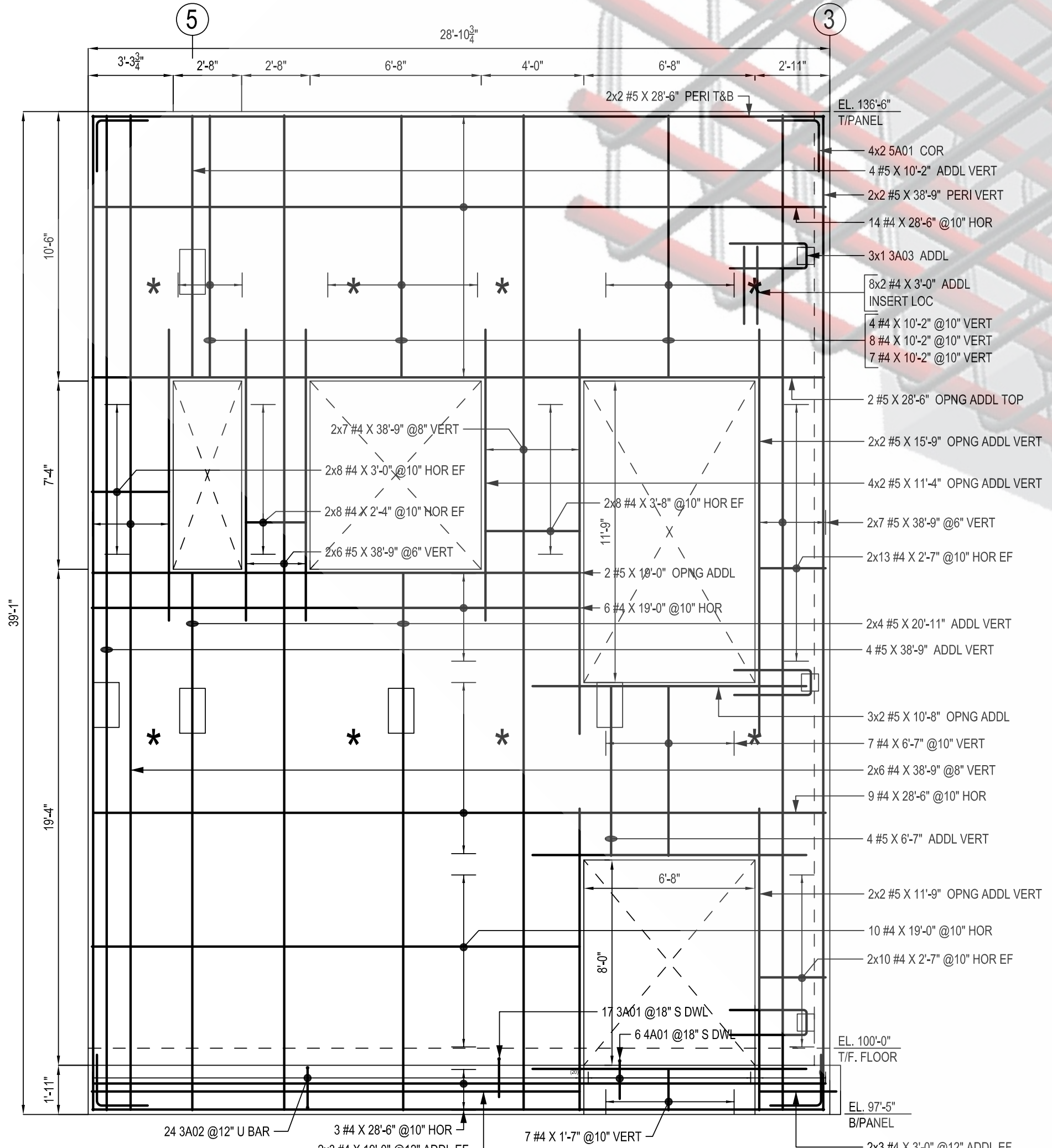
PANEL-P9 SCALE: 1/4"=1'-0" SDR: S2.01 & S3.11
