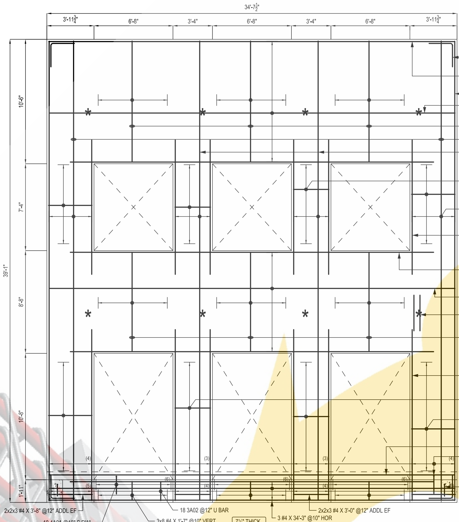
PANEL-P7 SCALE: 1/4"=1'-0" SDR: S2.01 & S3.11
